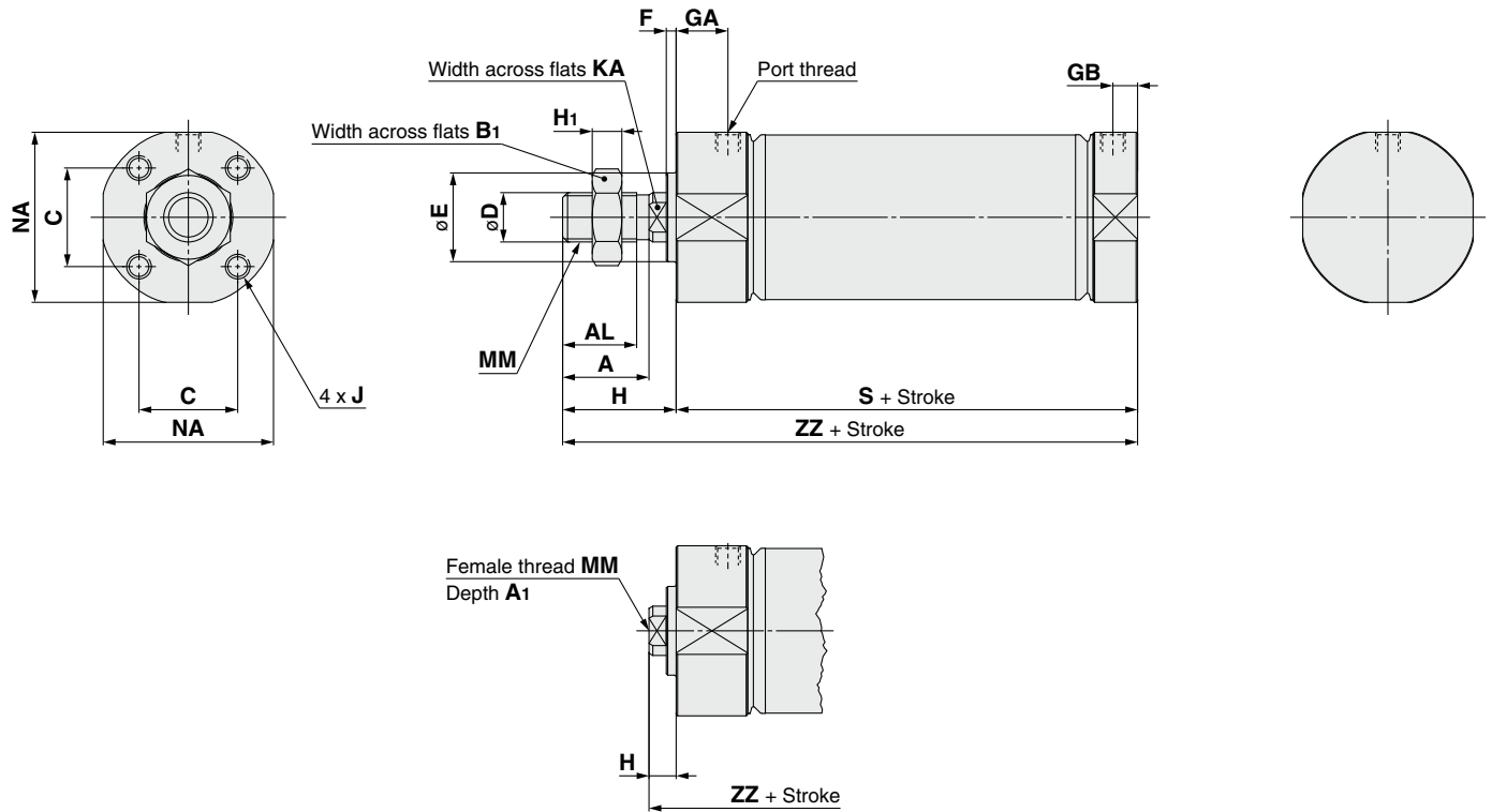
Female rod end
